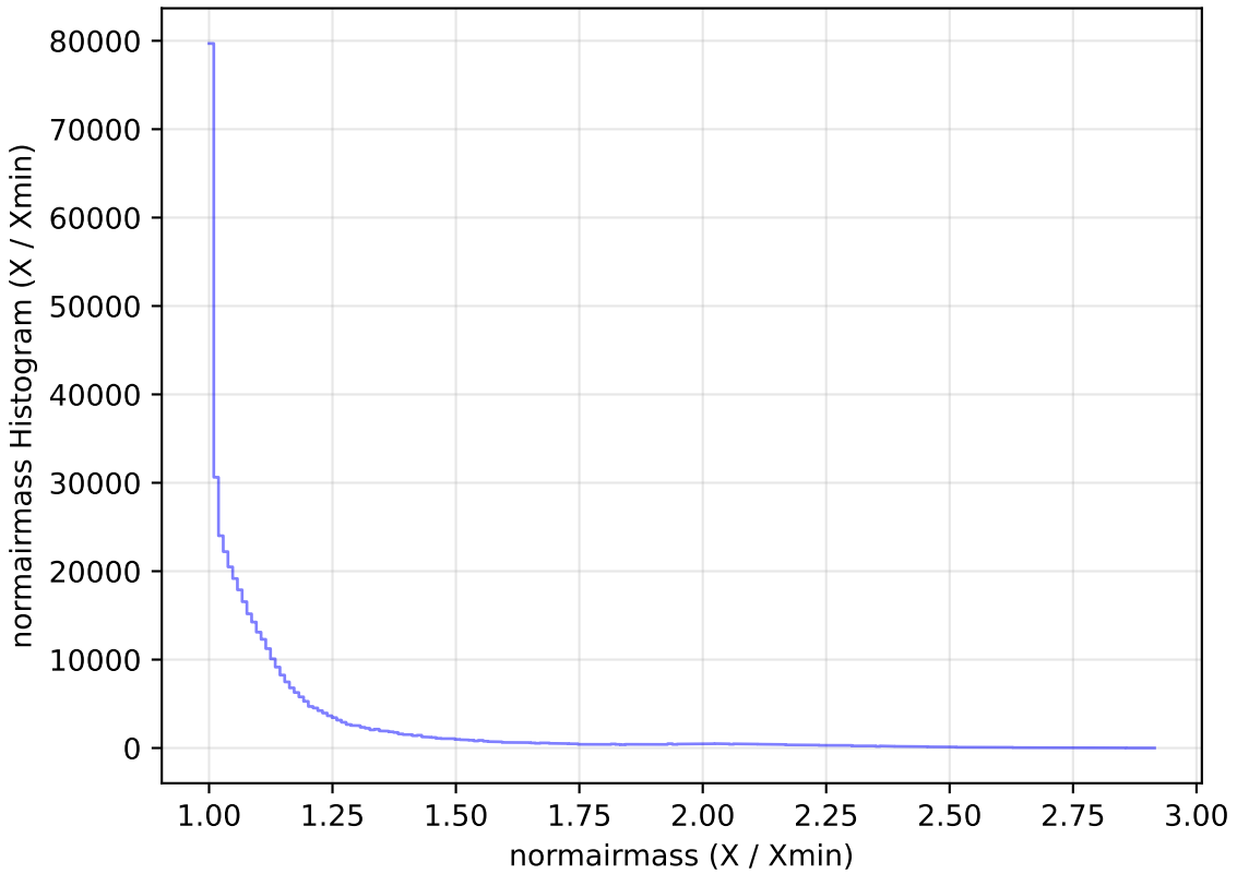
internal_u_expt45_nscale1.5v3.4_10yrs WFD i band: normairmass Histogram
