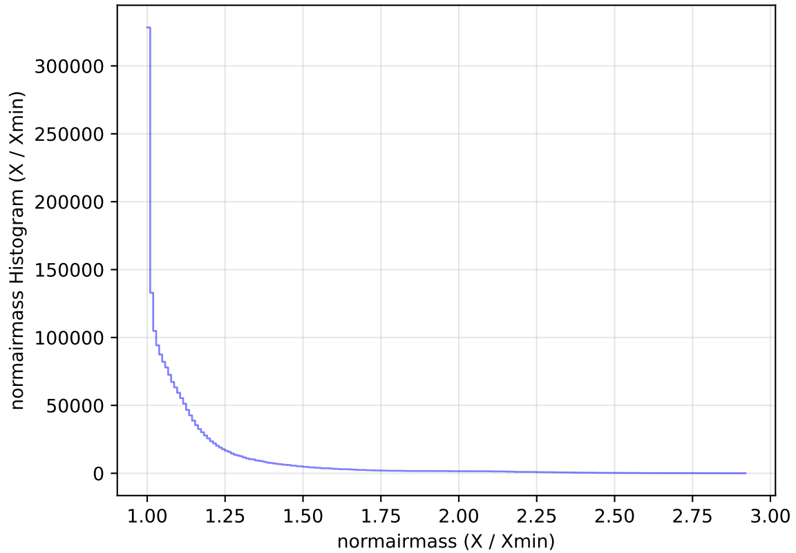
internal_u_expt45_nscale1.5v3.4_10yrs WFD all bands: normairmass Histogram
