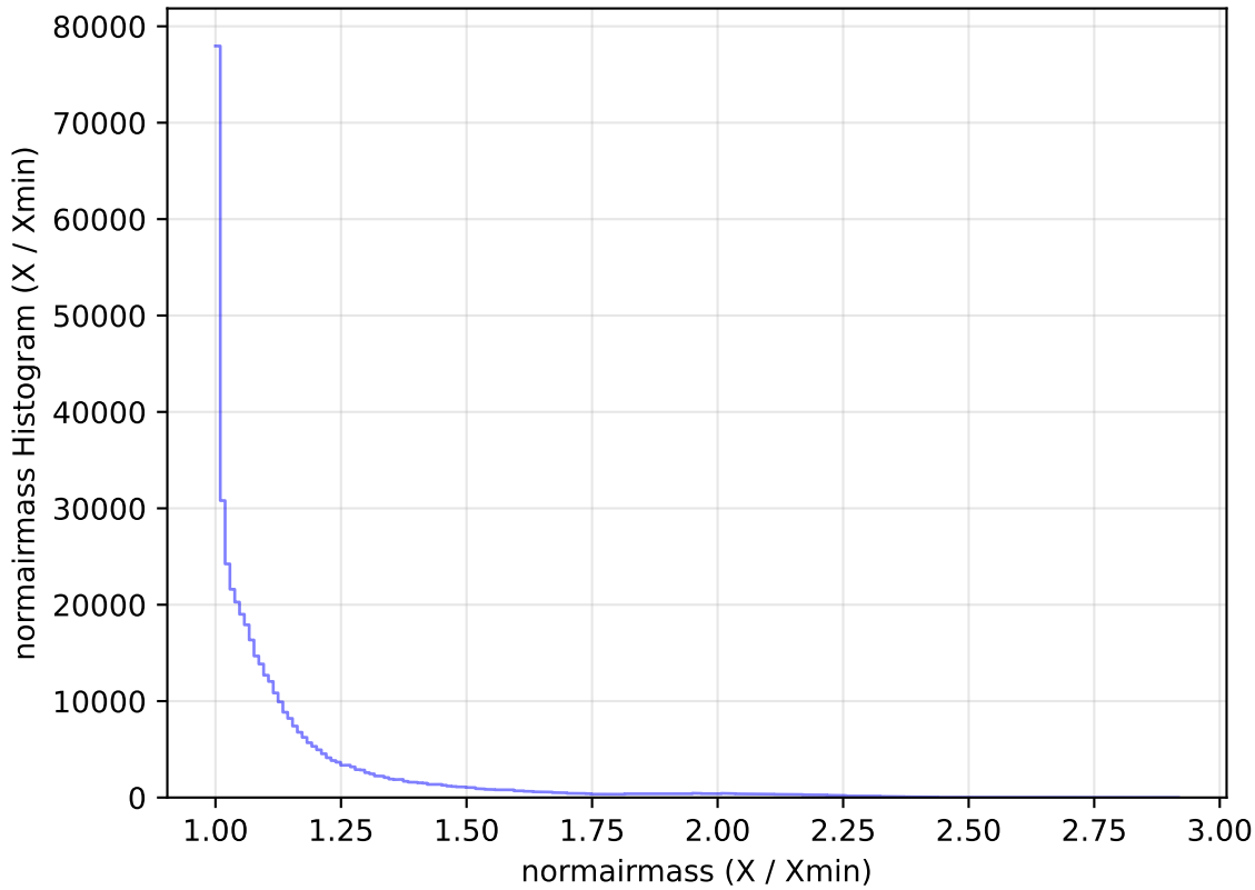
internal_u_expt45_nscale1.5v3.4_10yrs All sky r band: normairmass Histogram
