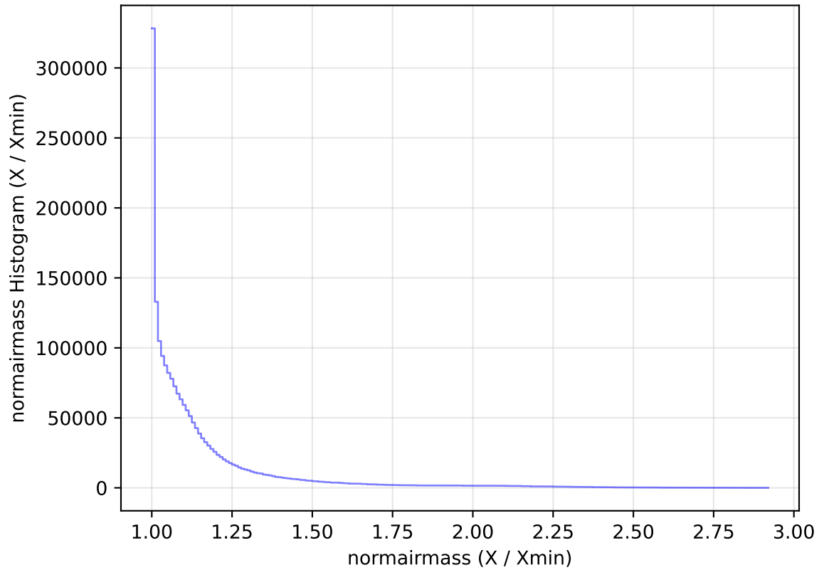
internal_u_expt45_nscale1.5v3.4_10yrs All sky all bands: normairmass Histogram
