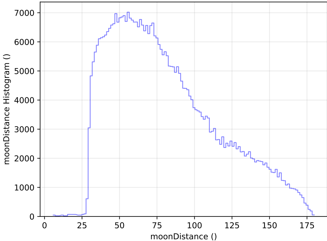
internal_u_expt45_nscale1.5v3.4_10yrs WFD z band: moonDistance Histogram
