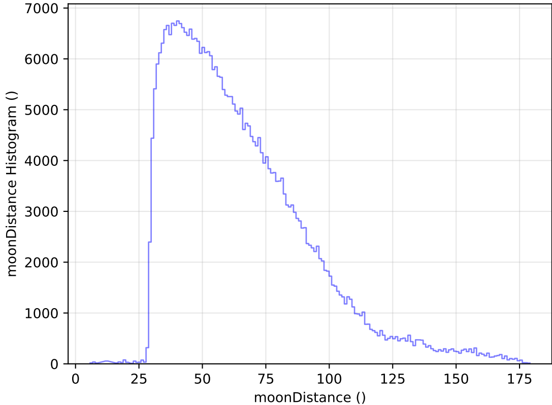
internal_u_expt45_nscale1.5v3.4_10yrs WFD y band: moonDistance Histogram
