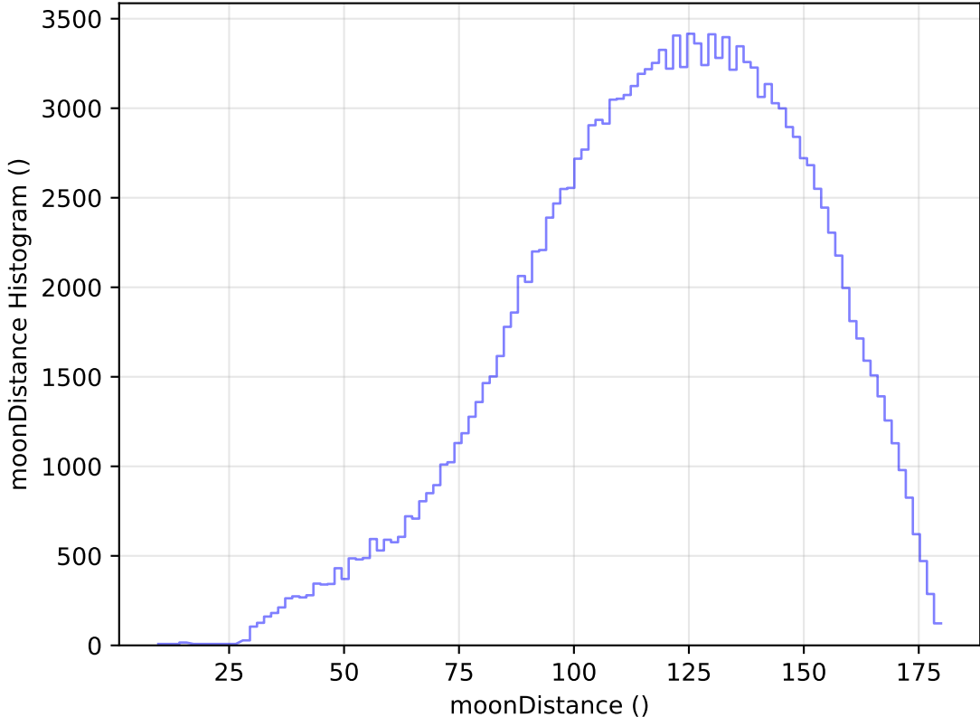
internal_u_expt45_nscale1.5v3.4_10yrs WFD u band: moonDistance Histogram
