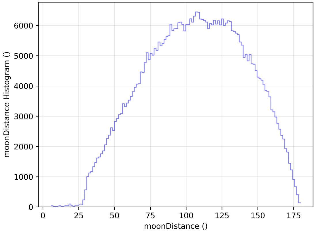
internal_u_expt45_nscale1.5v3.4_10yrs WFD r band: moonDistance Histogram
