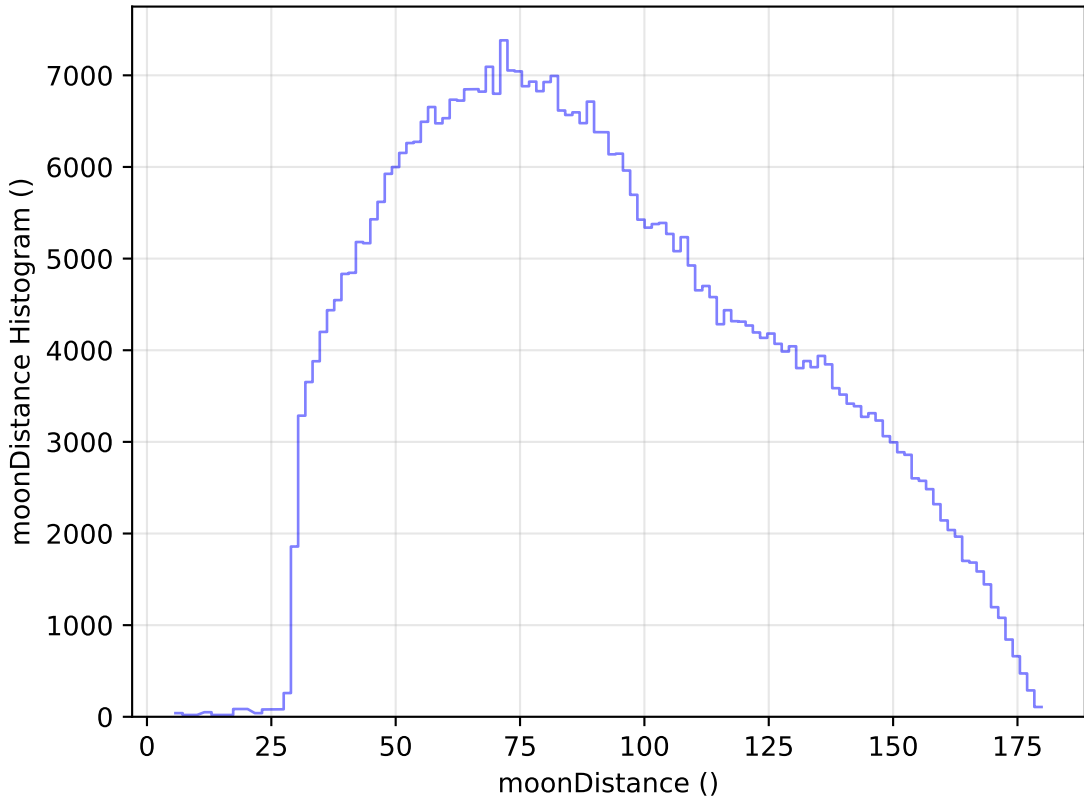
internal_u_expt45_nscale1.5v3.4_10yrs WFD i band: moonDistance Histogram
