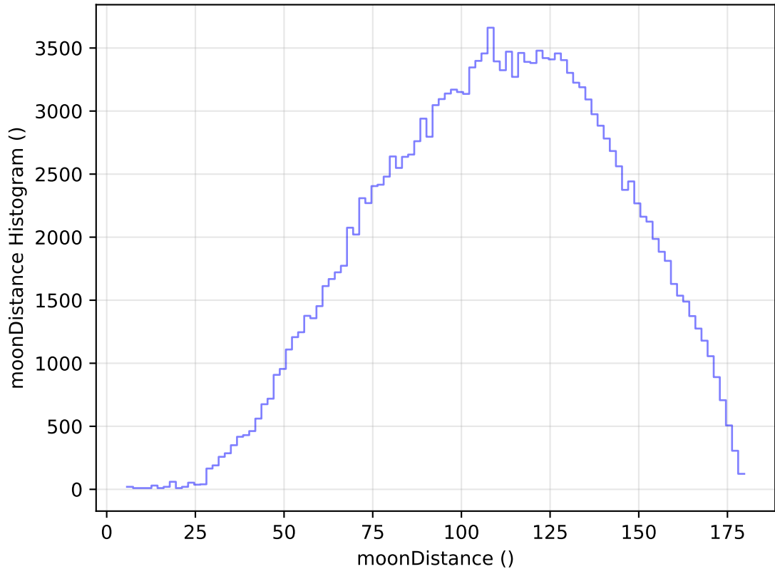
internal_u_expt45_nscale1.5v3.4_10yrs WFD g band: moonDistance Histogram
