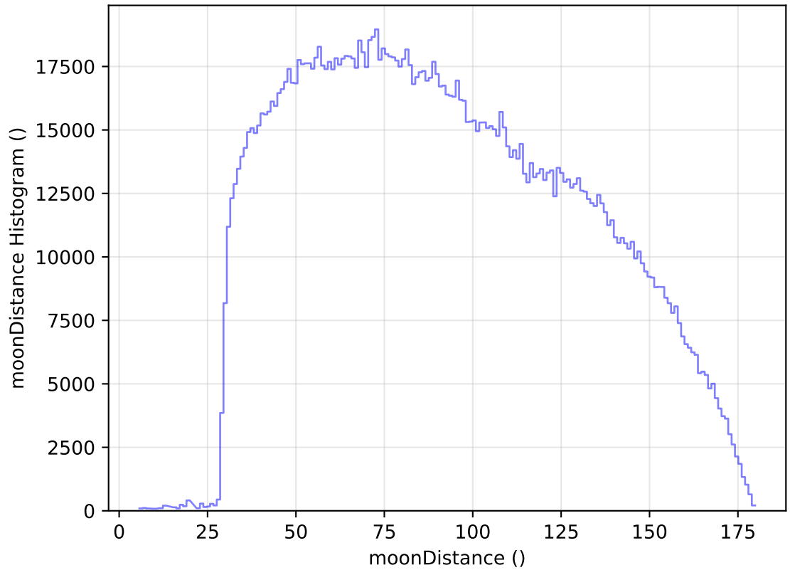
internal_u_expt45_nscale1.5v3.4_10yrs WFD all bands: moonDistance Histogram
