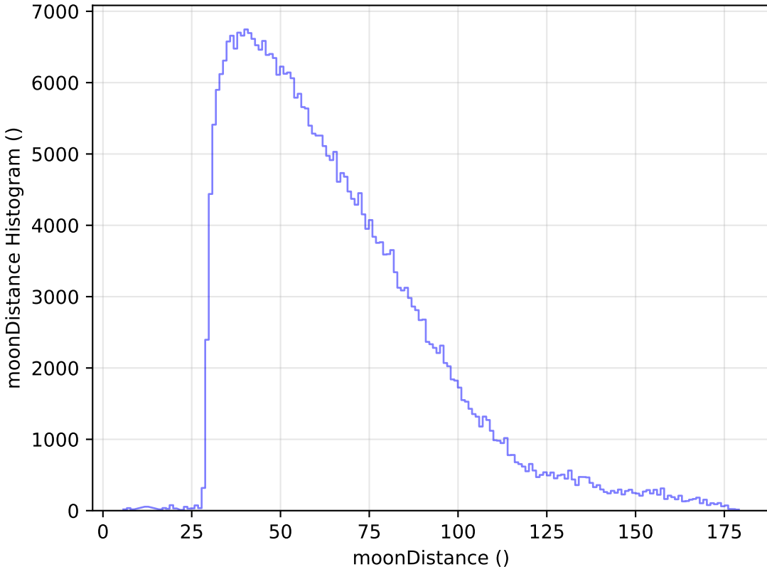
internal_u_expt45_nscale1.5v3.4_10yrs All sky y band: moonDistance Histogram
