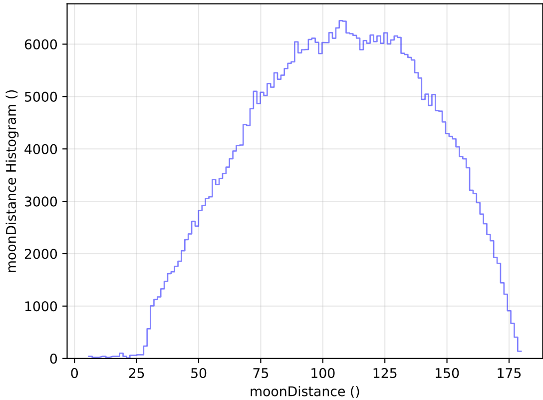
internal_u_expt45_nscale1.5v3.4_10yrs All sky r band: moonDistance Histogram
