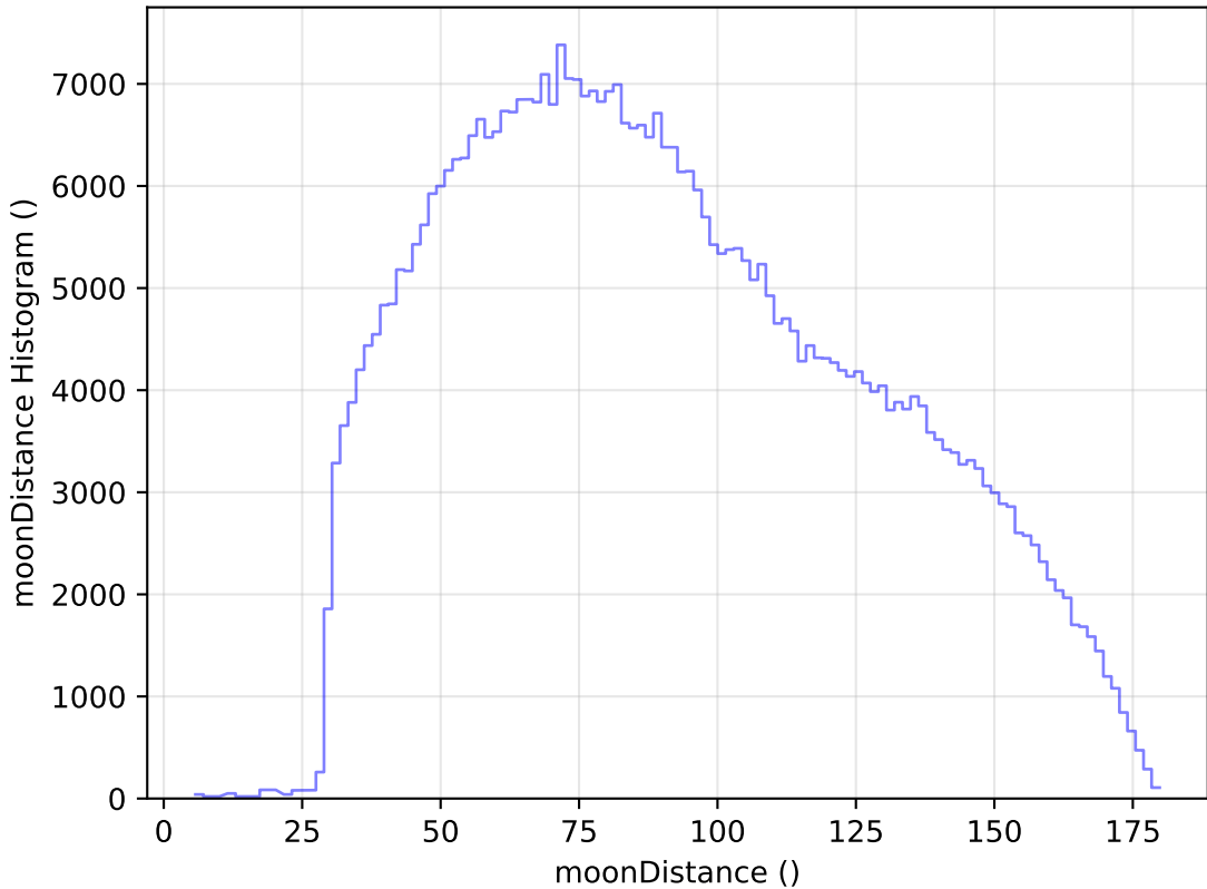
internal_u_expt45_nscale1.5v3.4_10yrs All sky i band: moonDistance Histogram
