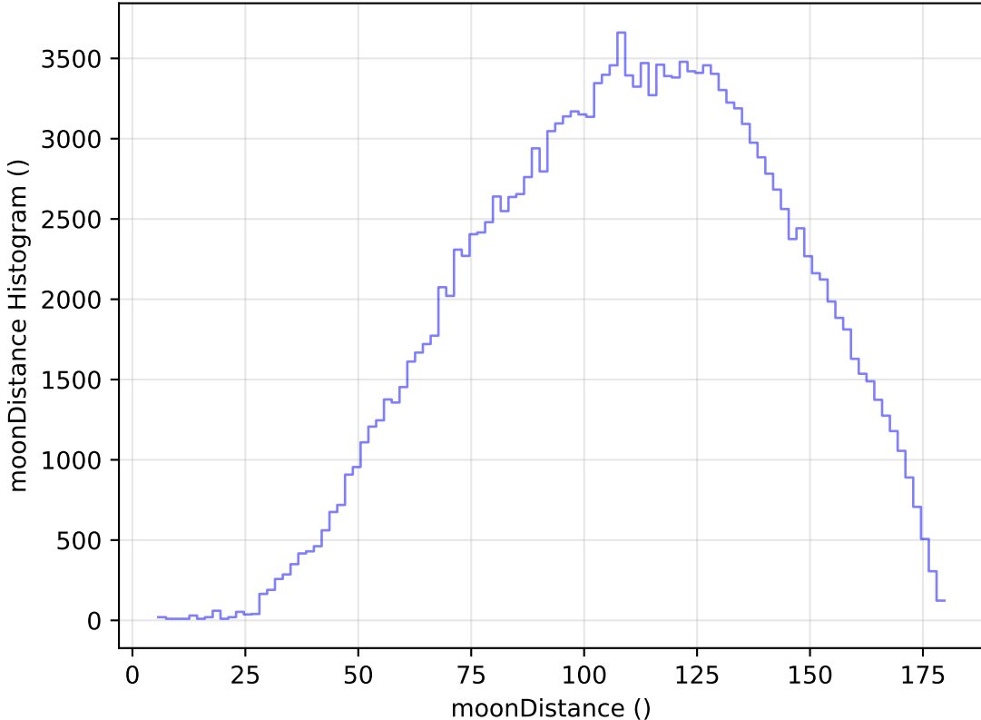
internal_u_expt45_nscale1.5v3.4_10yrs All sky g band: moonDistance Histogram
