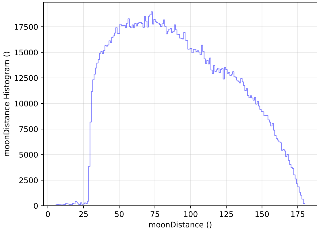
internal_u_expt45_nscale1.5v3.4_10yrs All sky all bands: moonDistance Histogram
