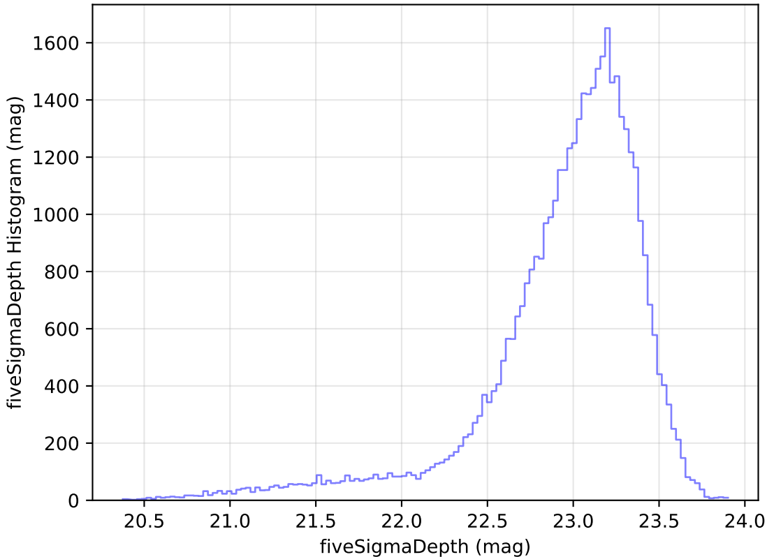
internal_u_expt45_nscale1.5v3.4_10yrs Yr 1 z band: fiveSigmaDepth Histogram
