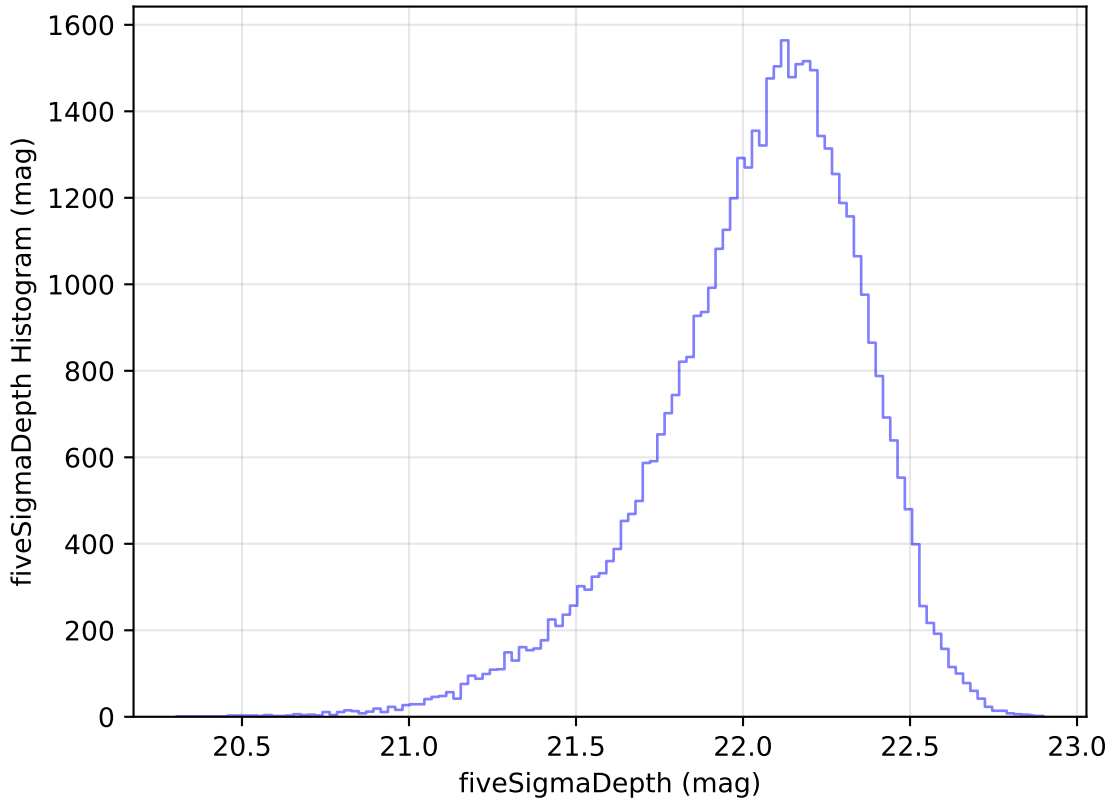
internal_u_expt45_nscale1.5v3.4_10yrs Yr 1 y band: fiveSigmaDepth Histogram
