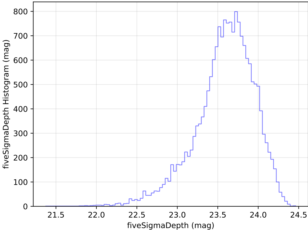
internal_u_expt45_nscale1.5v3.4_10yrs Yr 1 u band: fiveSigmaDepth Histogram
