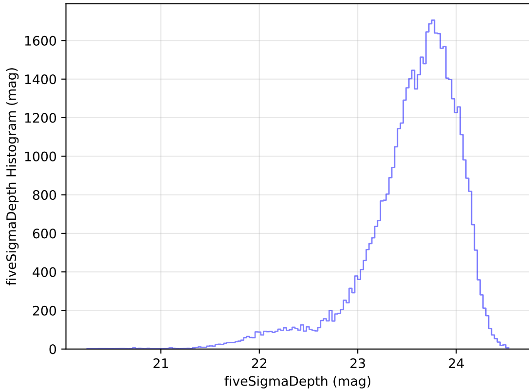
internal_u_expt45_nscale1.5v3.4_10yrs Yr 1 i band: fiveSigmaDepth Histogram
