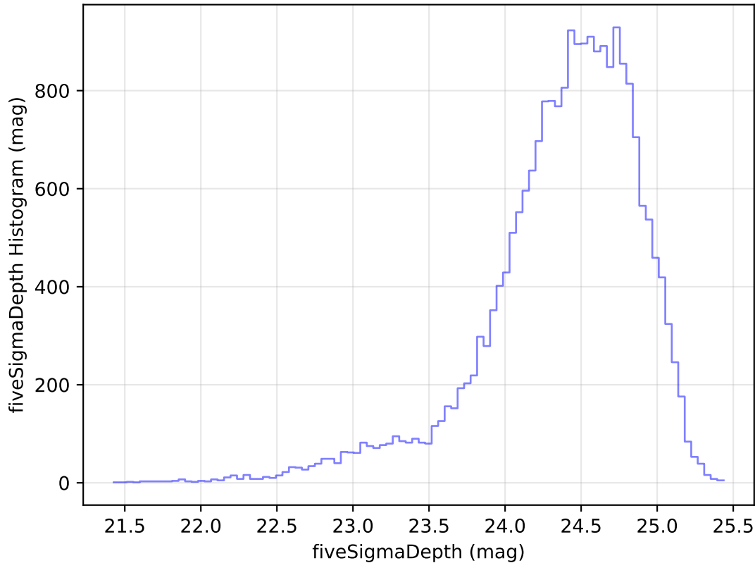
internal_u_expt45_nscale1.5v3.4_10yrs Yr 1 g band: fiveSigmaDepth Histogram
