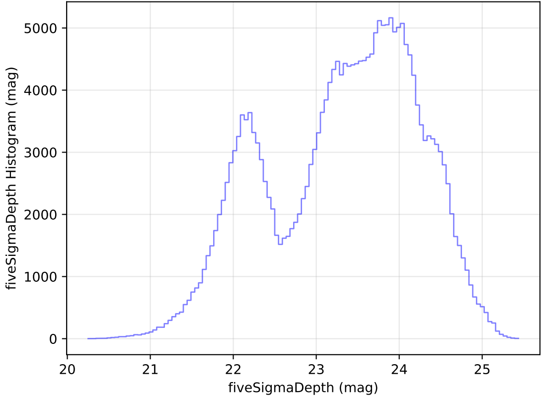
internal_u_expt45_nscale1.5v3.4_10yrs Yr 1 all bands: fiveSigmaDepth Histogram
