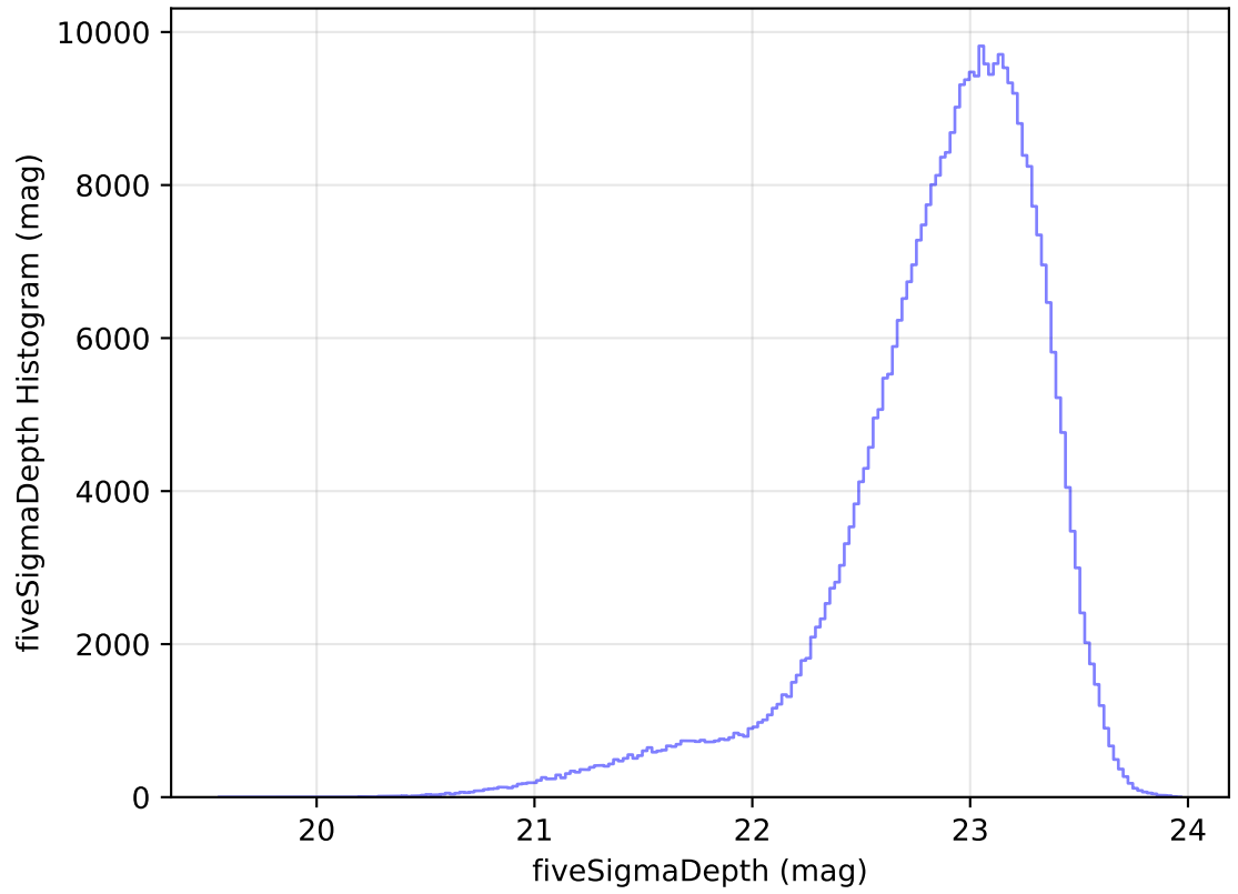
internal_u_expt45_nscale1.5v3.4_10yrs WFD z band: fiveSigmaDepth Histogram
