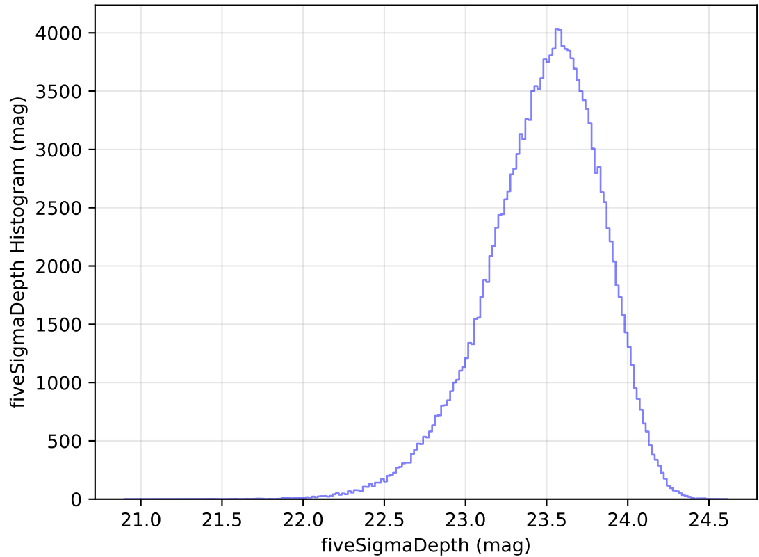
internal_u_expt45_nscale1.5v3.4_10yrs WFD u band: fiveSigmaDepth Histogram
