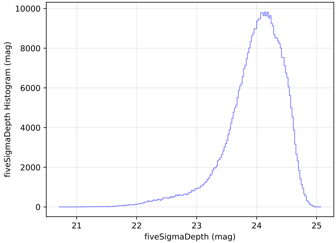
internal_u_expt45_nscale1.5v3.4_10yrs WFD r band: fiveSigmaDepth Histogram
