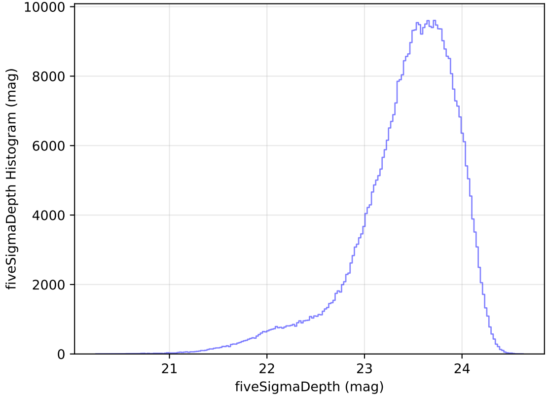
internal_u_expt45_nscale1.5v3.4_10yrs WFD i band: fiveSigmaDepth Histogram
