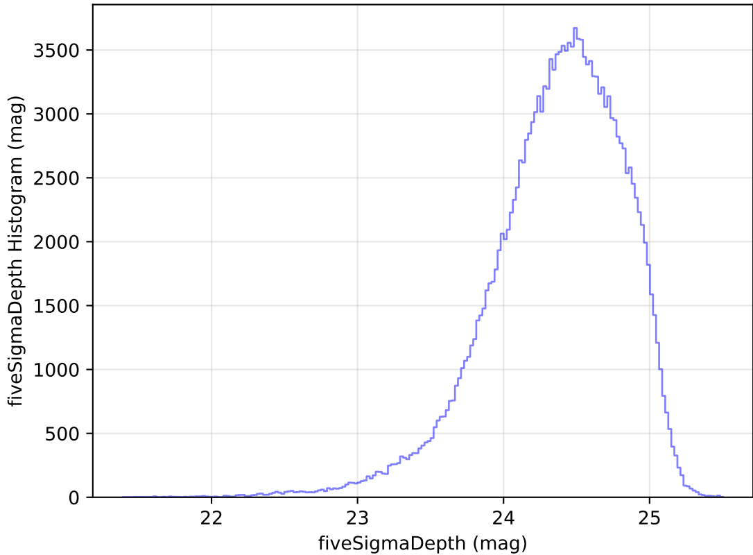
internal_u_expt45_nscale1.5v3.4_10yrs WFD g band: fiveSigmaDepth Histogram
