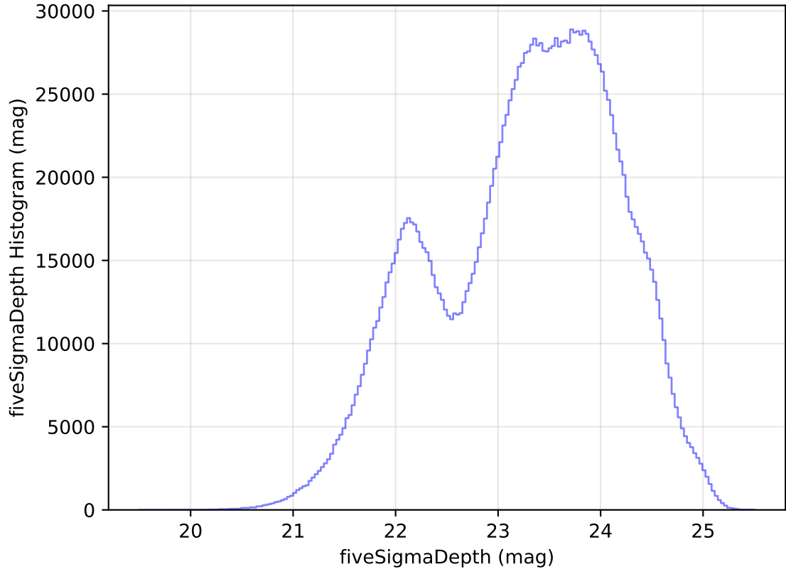
internal_u_expt45_nscale1.5v3.4_10yrs WFD all bands: fiveSigmaDepth Histogram
