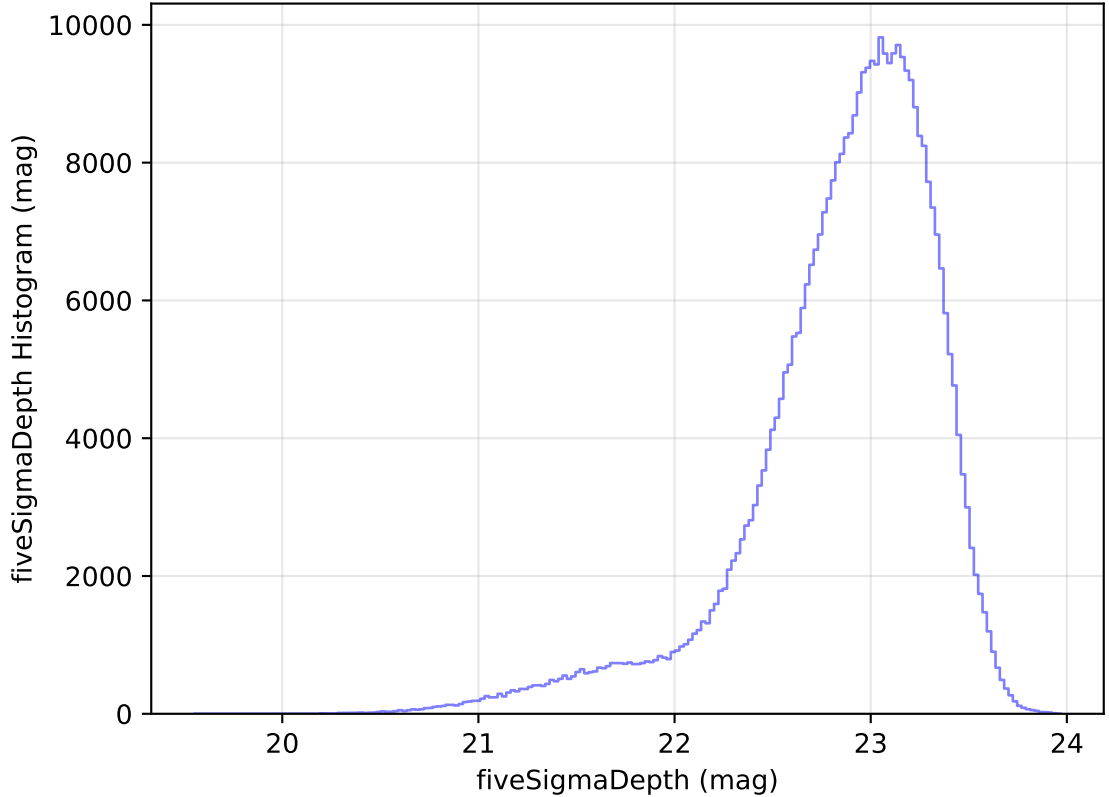
internal_u_expt45_nscale1.5v3.4_10yrs All sky z band: fiveSigmaDepth Histogram
