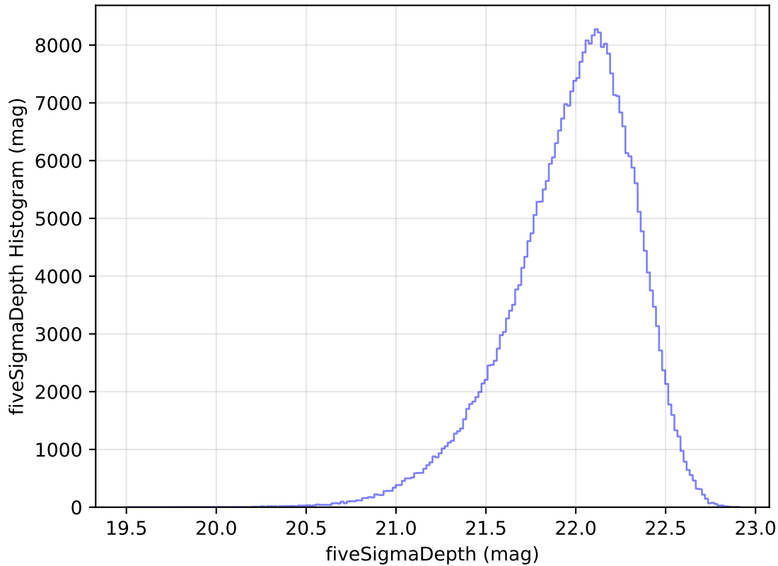
internal_u_expt45_nscale1.5v3.4_10yrs All sky y band: fiveSigmaDepth Histogram
