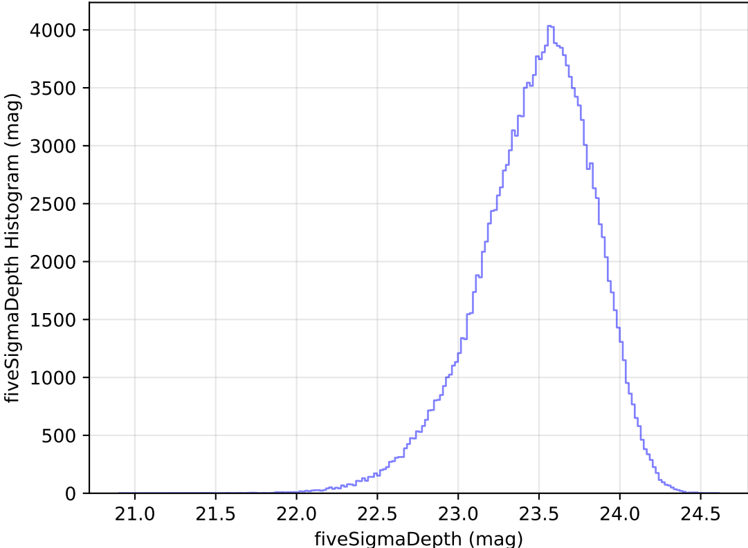
internal_u_expt45_nscale1.5v3.4_10yrs All sky u band: fiveSigmaDepth Histogram
