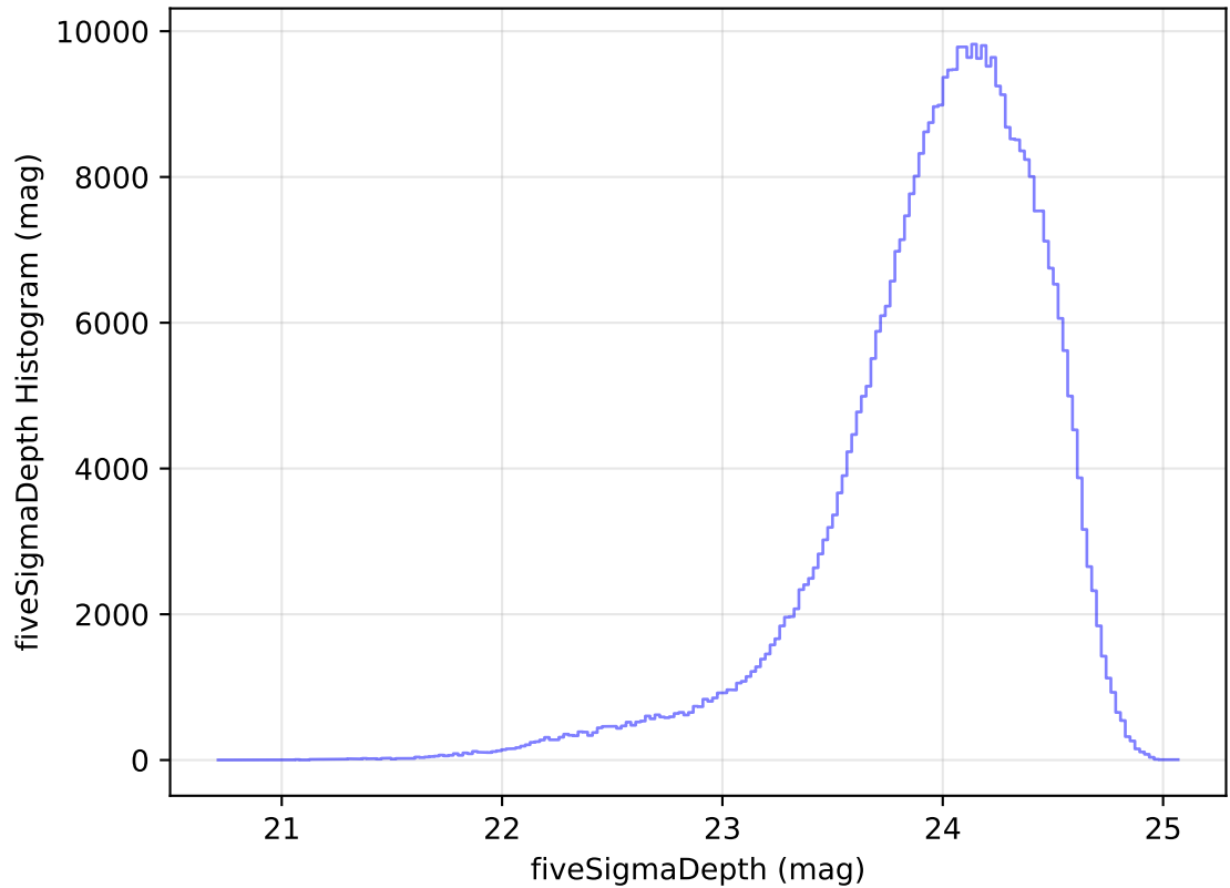
internal_u_expt45_nscale1.5v3.4_10yrs All sky r band: fiveSigmaDepth Histogram
