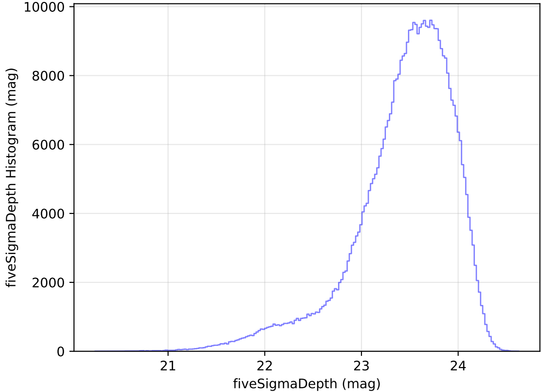
internal_u_expt45_nscale1.5v3.4_10yrs All sky i band: fiveSigmaDepth Histogram
