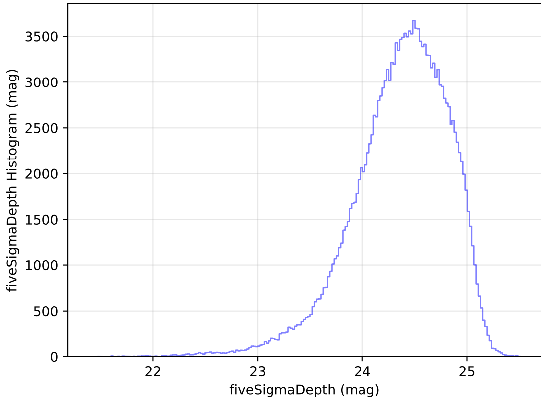
internal_u_expt45_nscale1.5v3.4_10yrs All sky g band: fiveSigmaDepth Histogram
