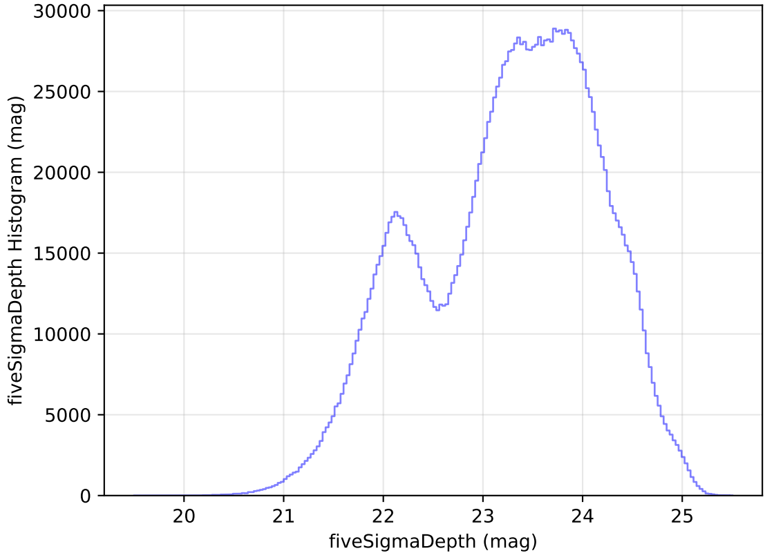
internal_u_expt45_nscale1.5v3.4_10yrs All sky all bands: fiveSigmaDepth Histogram
