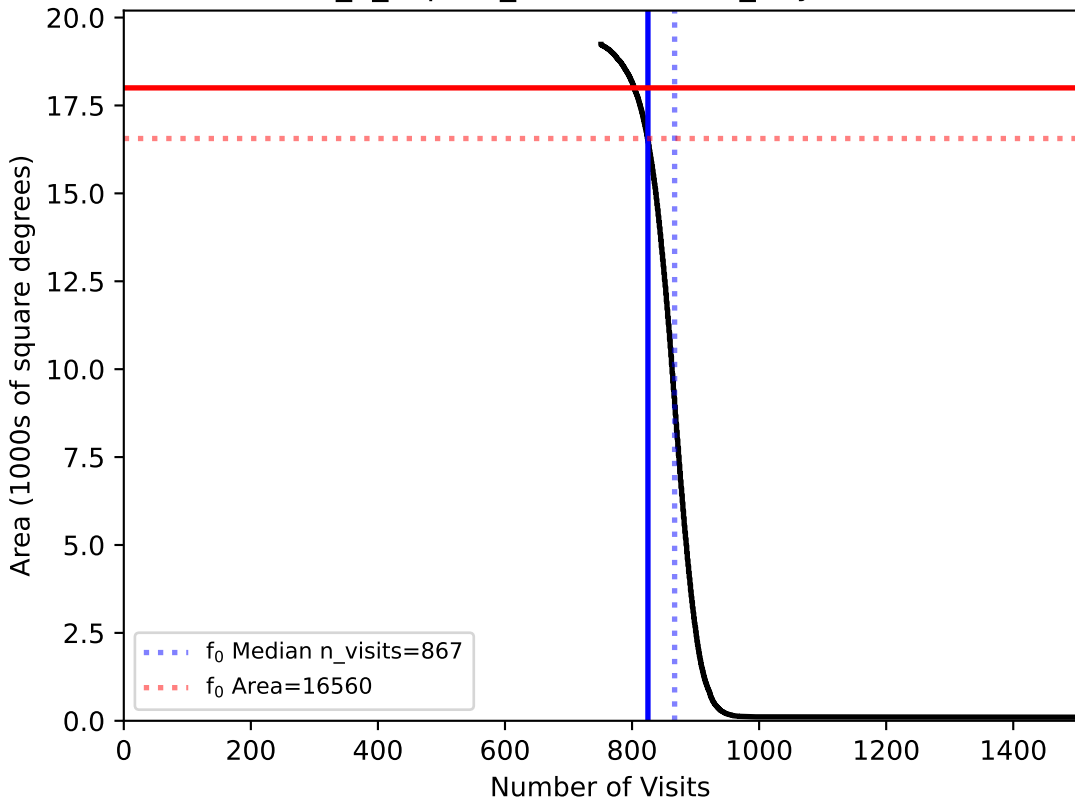
internal_u_expt45_nscale1.5v3.4_10yrs WFD: fO
