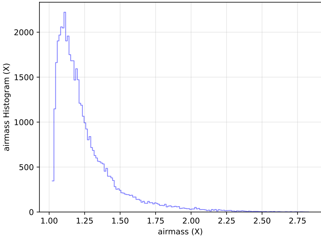
internal_u_expt45_nscale1.5v3.4_10yrs Yr 1 y band: airmass Histogram
