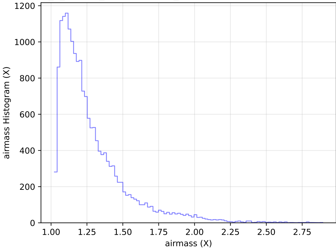
internal_u_expt45_nscale1.5v3.4_10yrs Yr 1 u band: airmass Histogram
