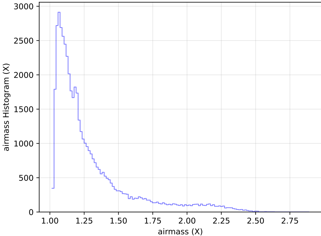
internal_u_expt45_nscale1.5v3.4_10yrs Yr 1 r band: airmass Histogram
