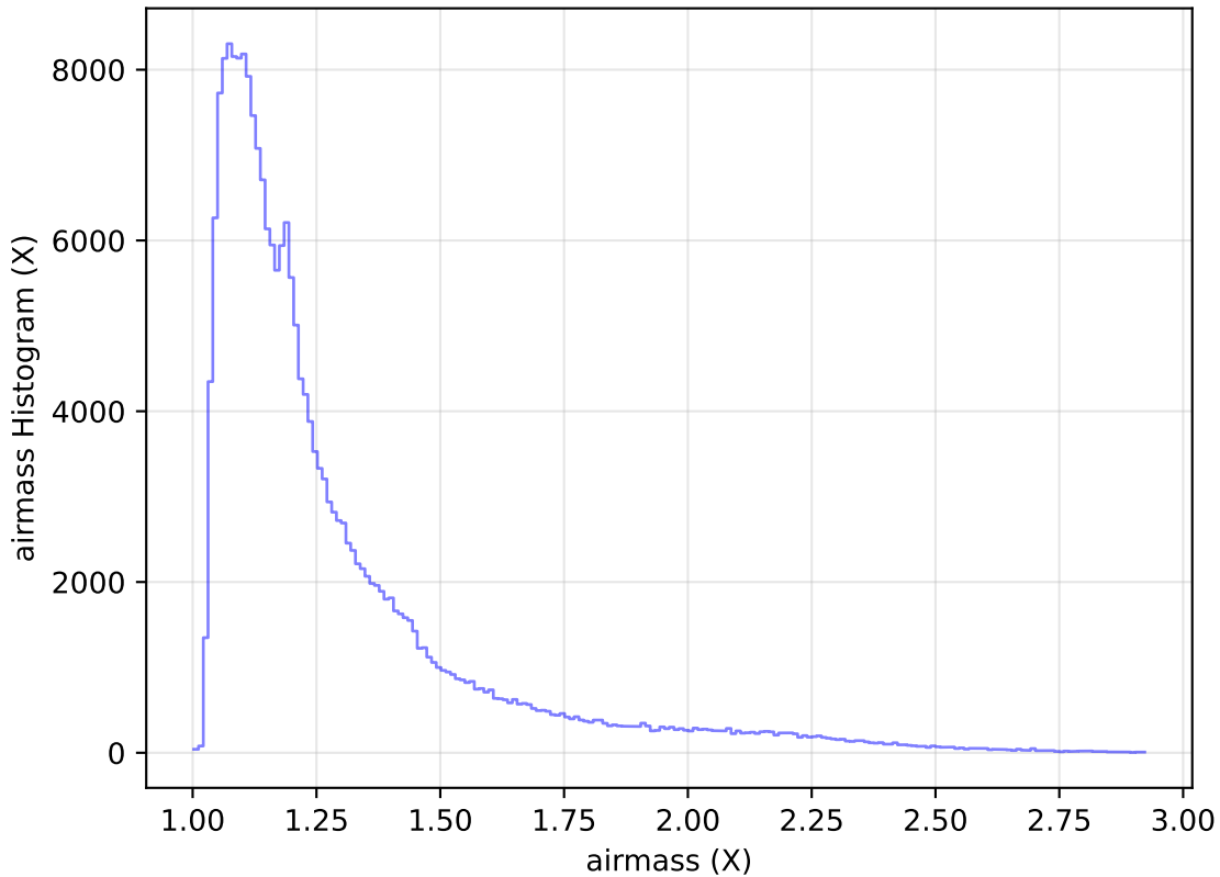
internal_u_expt45_nscale1.5v3.4_10yrs Yr 1 all bands: airmass Histogram
