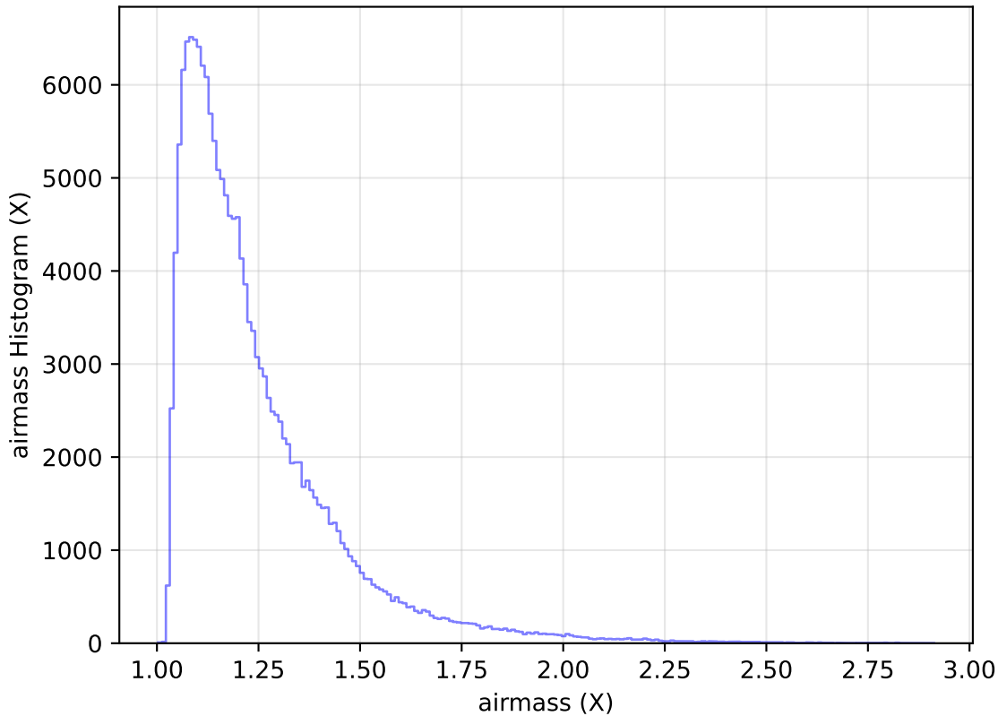
internal_u_expt45_nscale1.5v3.4_10yrs WFD u band: airmass Histogram
