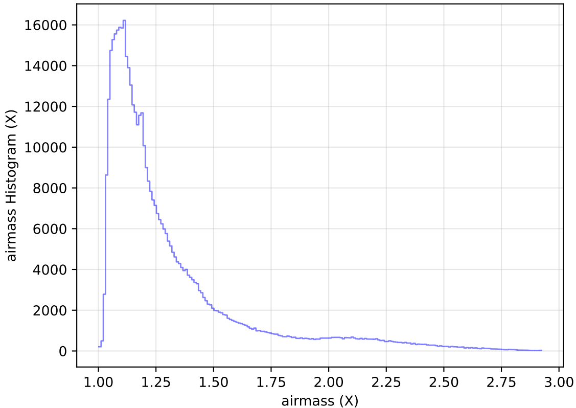
internal_u_expt45_nscale1.5v3.4_10yrs WFD i band: airmass Histogram
