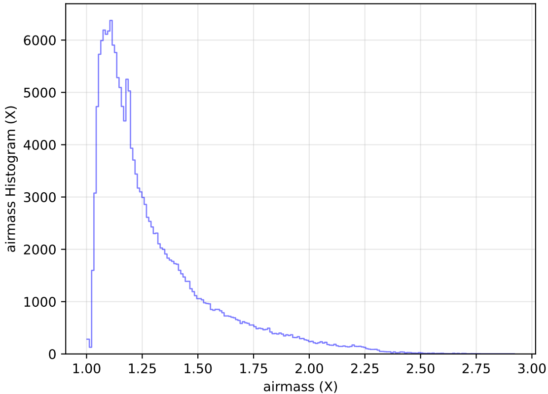
internal_u_expt45_nscale1.5v3.4_10yrs WFD g band: airmass Histogram
