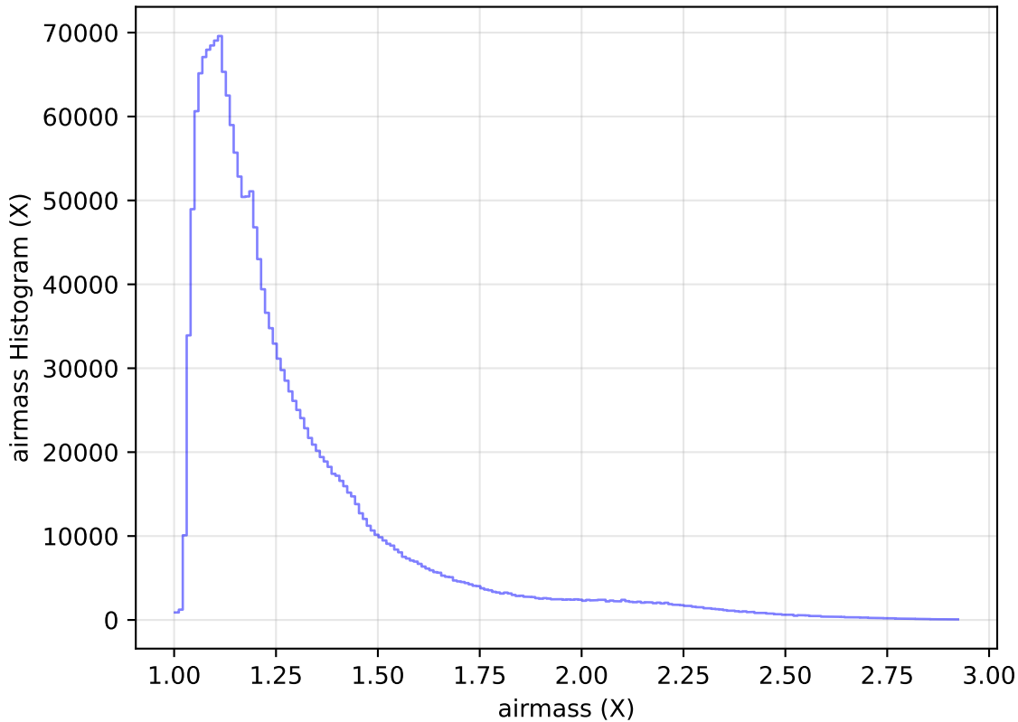
internal_u_expt45_nscale1.5v3.4_10yrs WFD all bands: airmass Histogram
