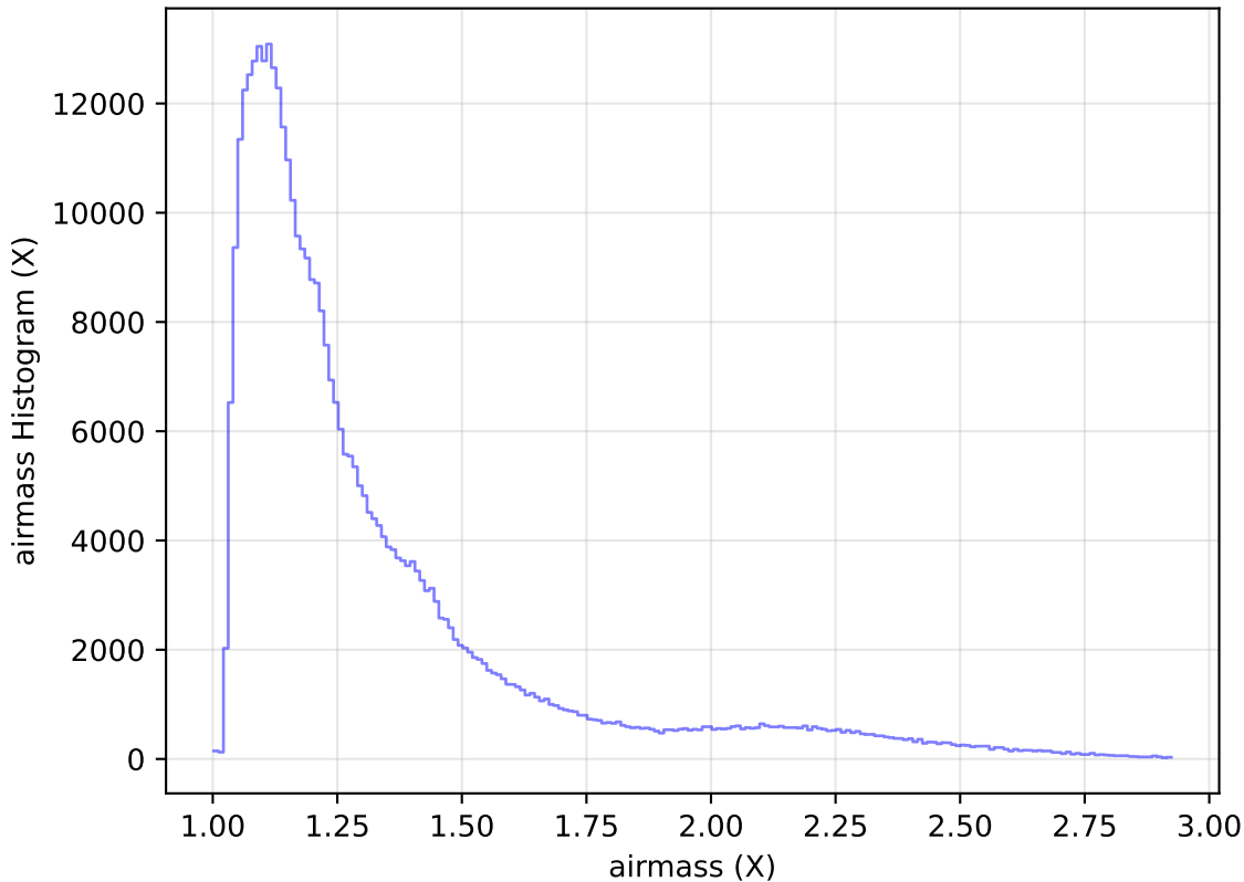
internal_u_expt45_nscale1.5v3.4_10yrs All sky z band: airmass Histogram
