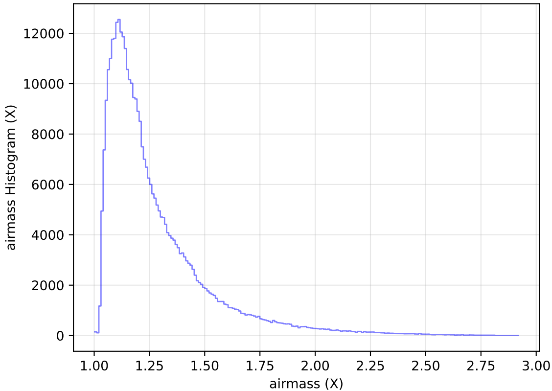
internal_u_expt45_nscale1.5v3.4_10yrs All sky y band: airmass Histogram
