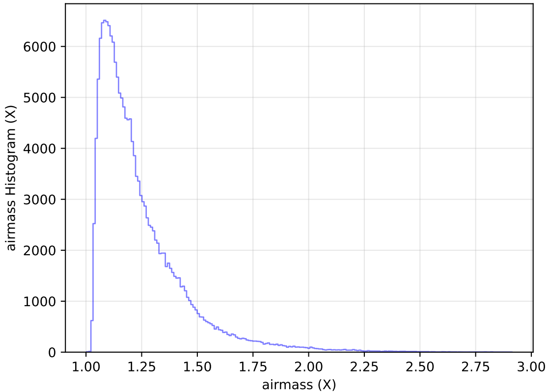
internal_u_expt45_nscale1.5v3.4_10yrs All sky u band: airmass Histogram
