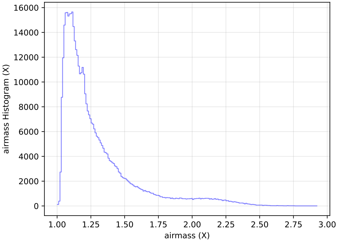
internal_u_expt45_nscale1.5v3.4_10yrs All sky r band: airmass Histogram
