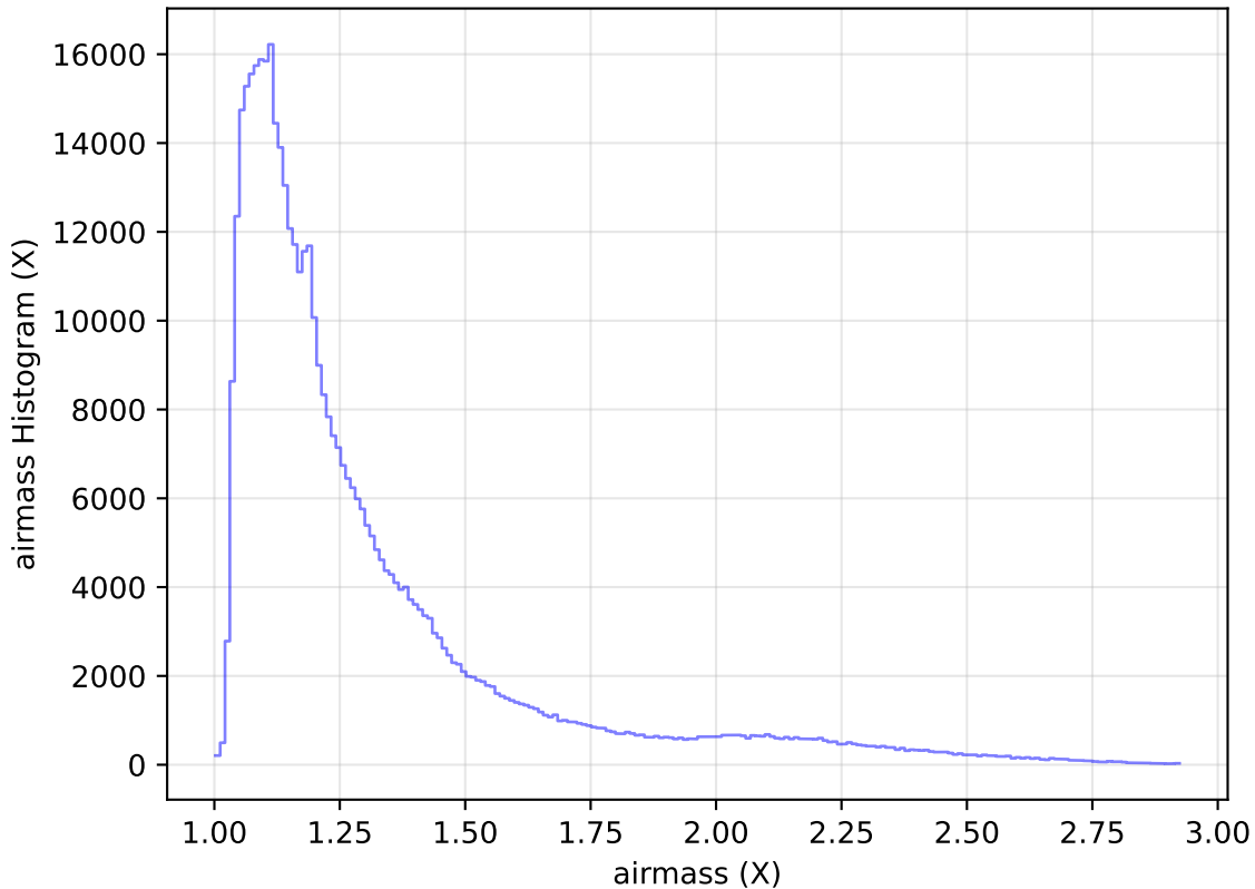
internal_u_expt45_nscale1.5v3.4_10yrs All sky i band: airmass Histogram
