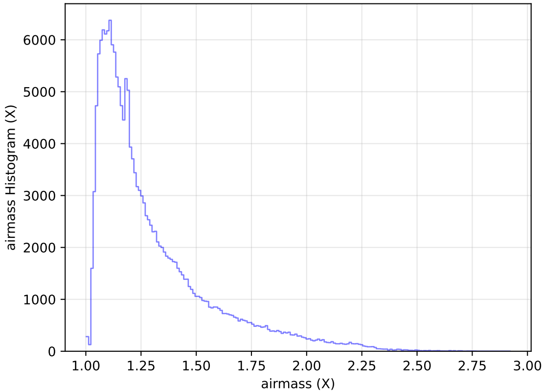
internal_u_expt45_nscale1.5v3.4_10yrs All sky g band: airmass Histogram
